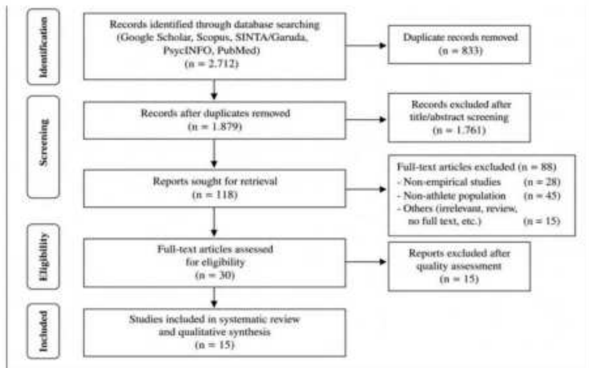
Gambar 1. PRISMA Diagram
